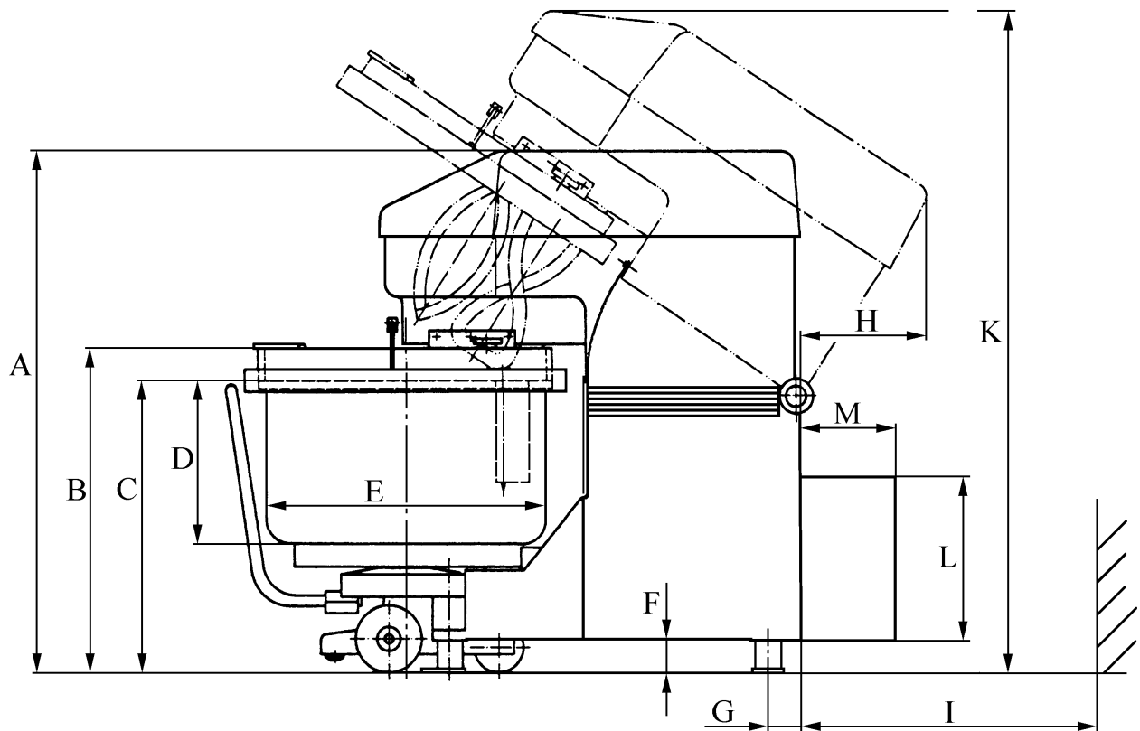
Fig. 2-2: Dimensions - Seen from the side -
